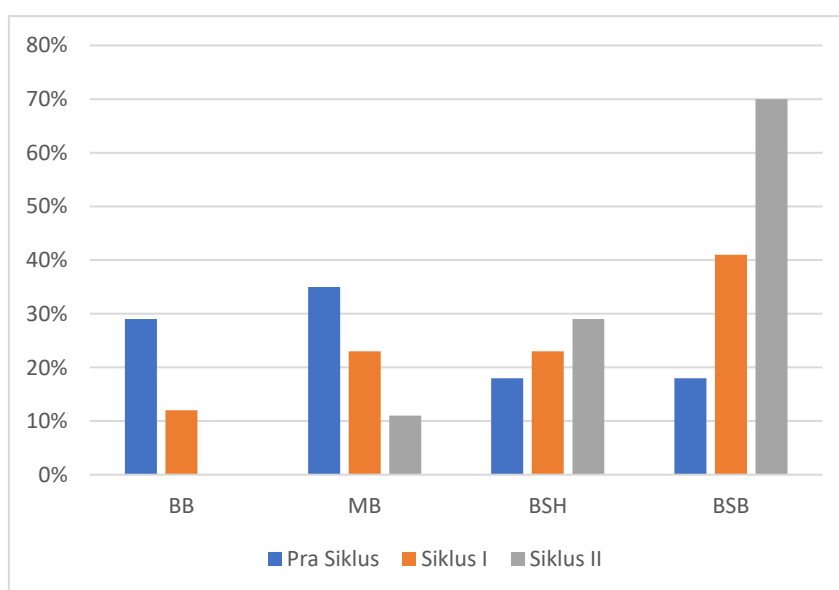
Gambar 4. 1 Diagram batang
