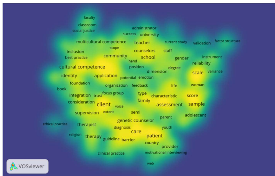
Gambar 3. Density Visualization
