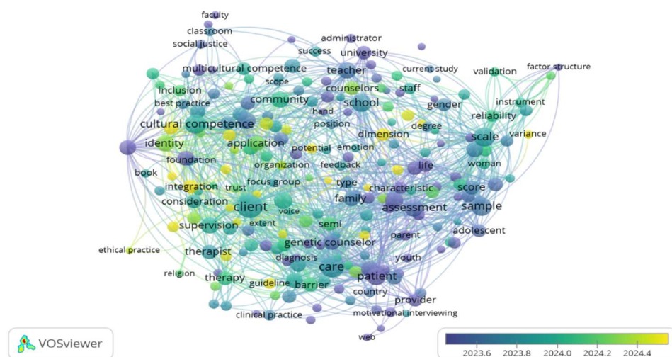
Gambar 2. Overlay Visualization
