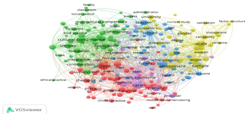
Gambar 1. Network Visualization
